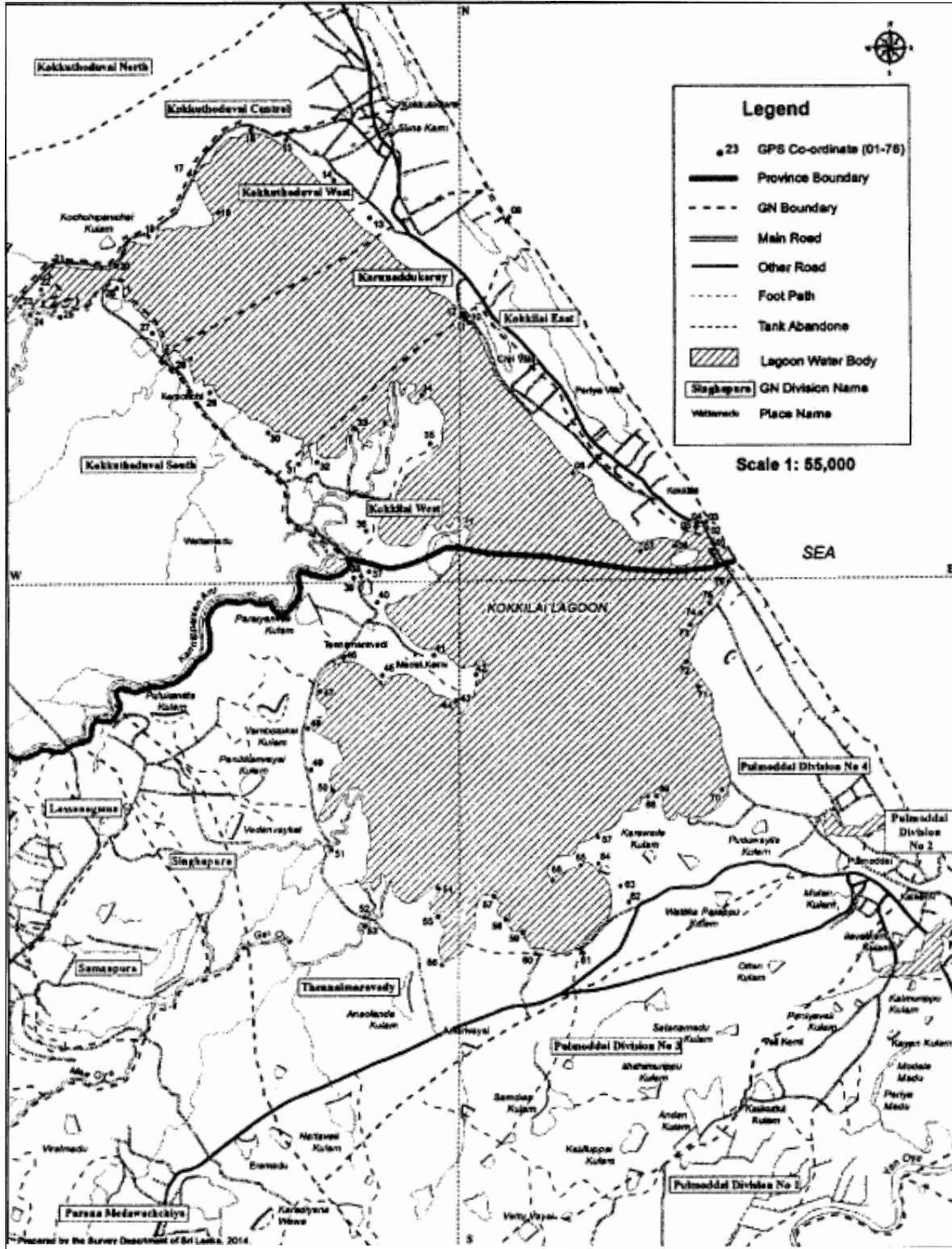
Map of Kokkilai Lagoon Fisheries Management Area
